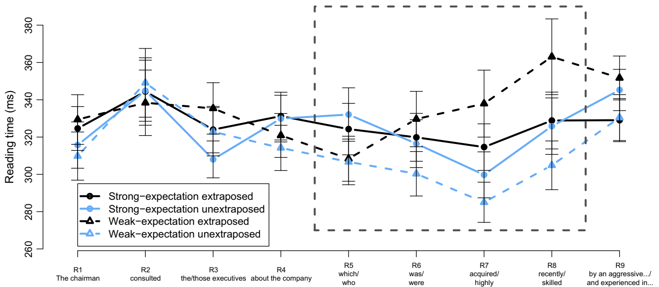
Fig. 6. Region-by-region reading times for Experiment 3.
