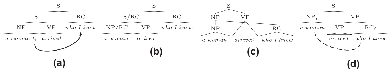
Fig. 1. Different phrase-structure representations for the non-projective dependency structure in (2b). In (a), the non-projective dependency is characterized by movement from an NP-internal trace. In (b), the non-projective dependency is represented by the missing-RC information transmitted between the NP and the top S categories. In (c), non-projectivity is directly represented as a discontinuous constituent. In (d), non-projectivity is represented as a special syntactic coindexing relation between a base-generated RC and the NP it modifies.
