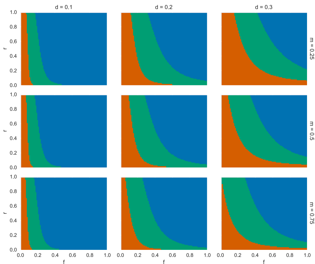
Fig. 4. Regions of different model behavior regarding structural forgetting in terms of the free parameters d (noise rate), m (postnominal modification rate), r (relative clause rate), and f (verb-final relative clause rate). \blacksquare = U_1U_2 , \blacksquare = G_1U_2 (like English), \blacksquare = G_1G_2 (like German; see text).
