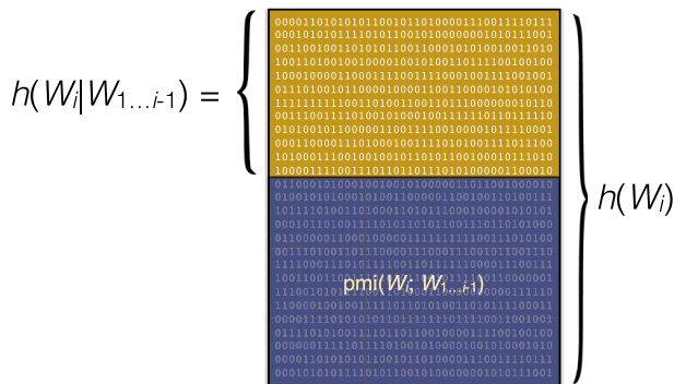
Fig. 6. Relation of conditional surprisal h(w_i|w_1, \dots, w_{i-1}) , unconditional surprisal h(w_i) , and pointwise mutual information \text{pmi}(w_i; w_1, \dots, w_{i-1}) .
